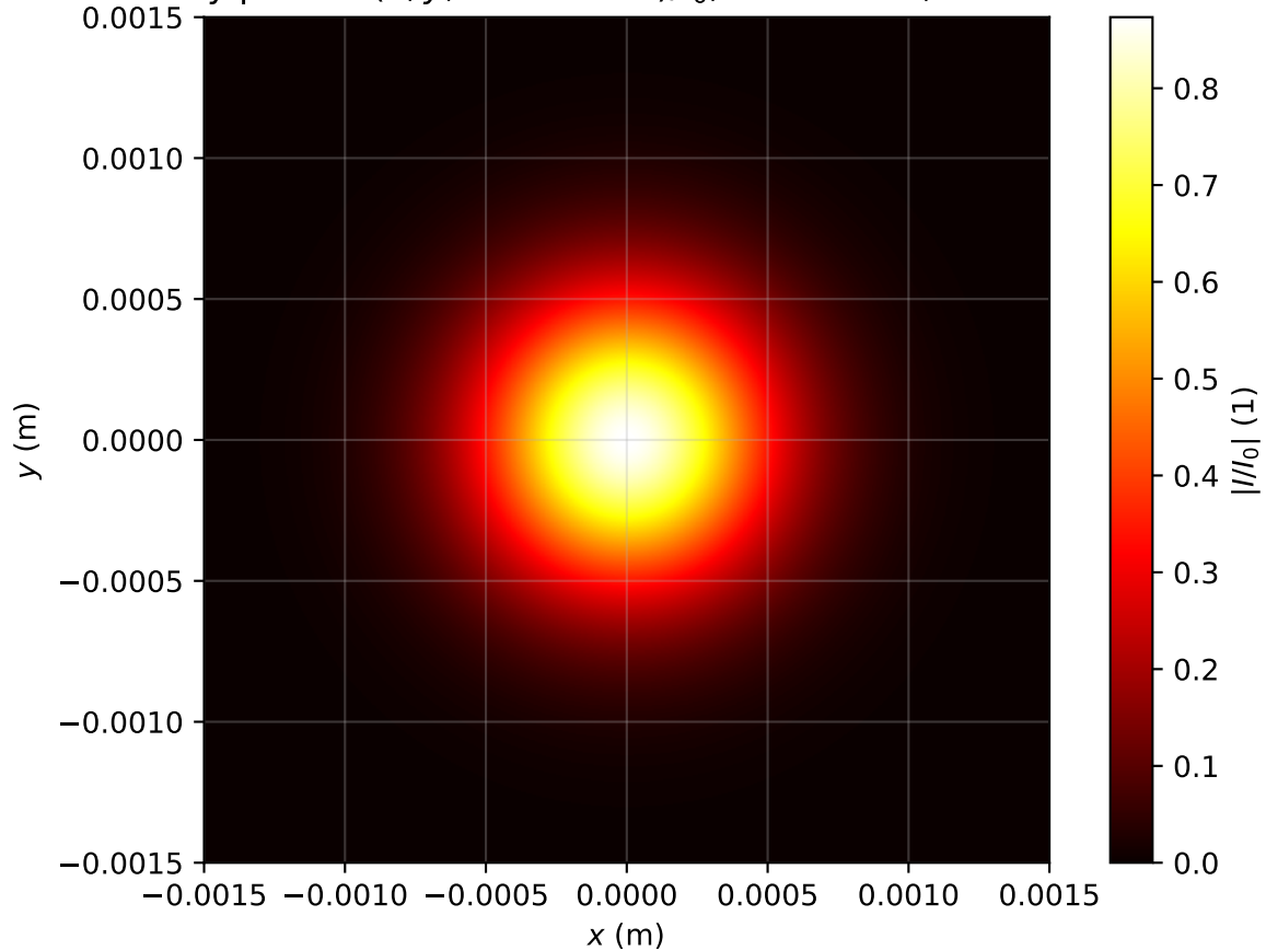
Intensity profile I(x, y, z = 1.035m)/I_0 , Pin=0.2Pcr, artificial time
